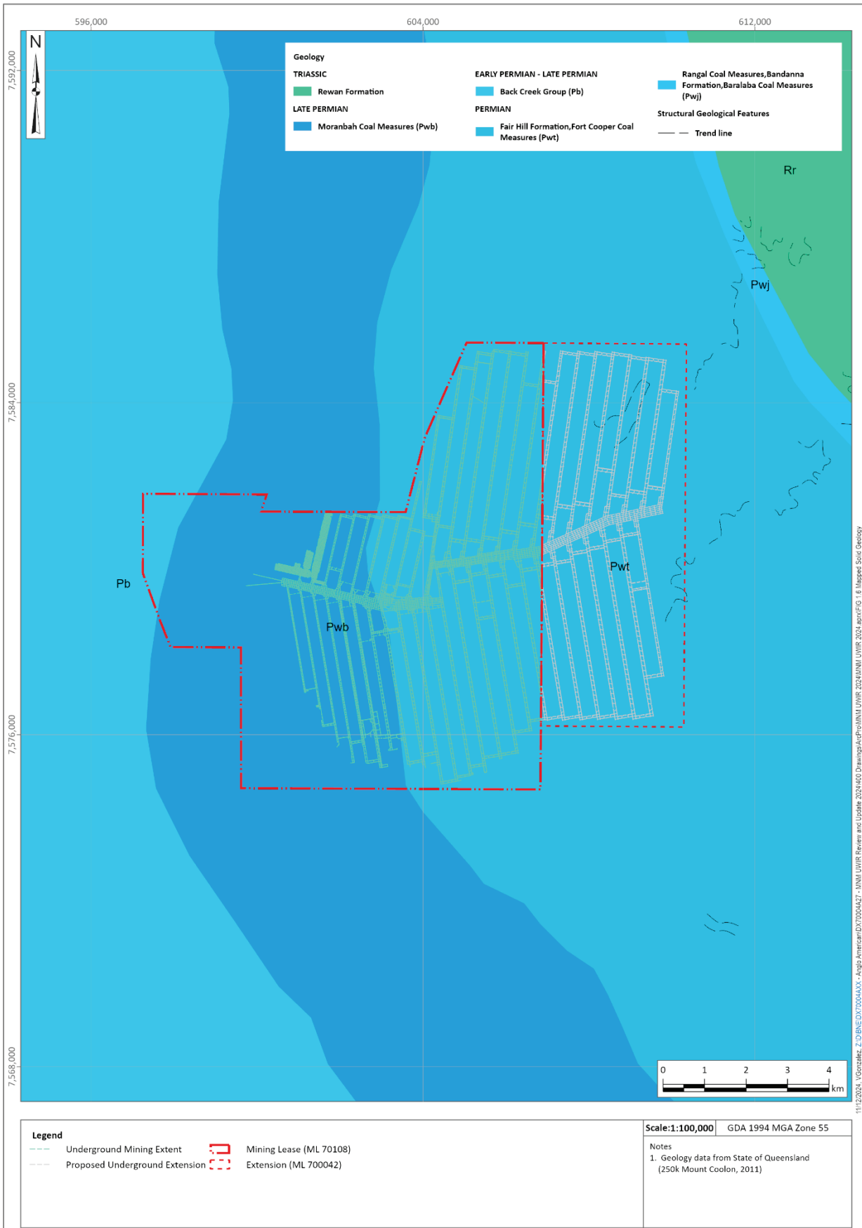
Figure 5.2 Mapped Solid (Regional) Geology (State of Queensland, 2024c)
