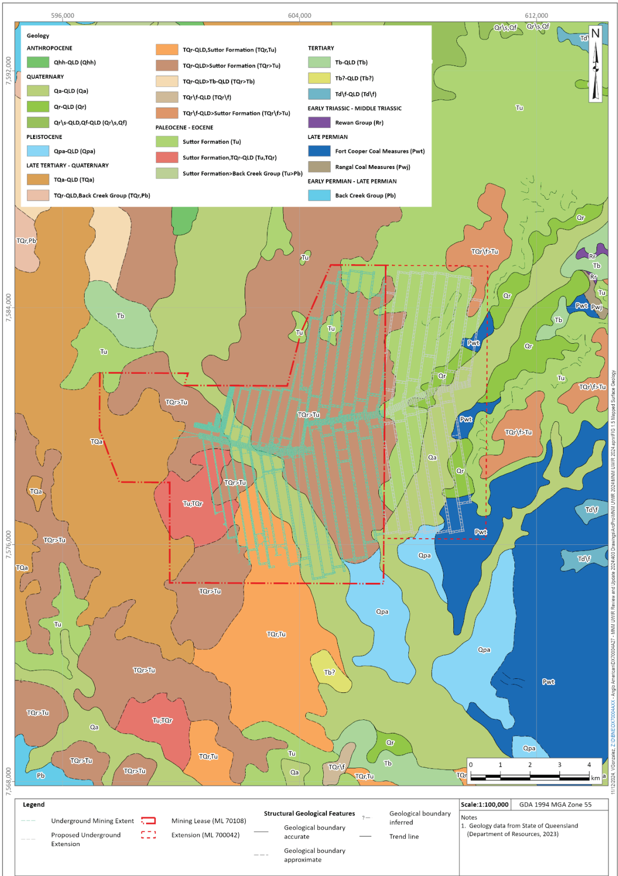
Figure 5.1 Mapped Surface Geology (State of Queensland, 2024c)
